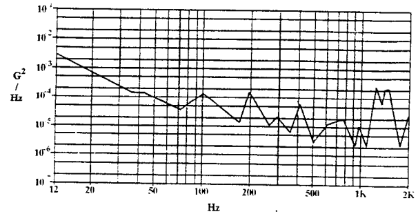
Figure 3. Exaggerated Shaker drive PSD resulting from amplitude edited field data.
