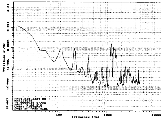
Figure 2. Ensemble averaged PSD from service records
